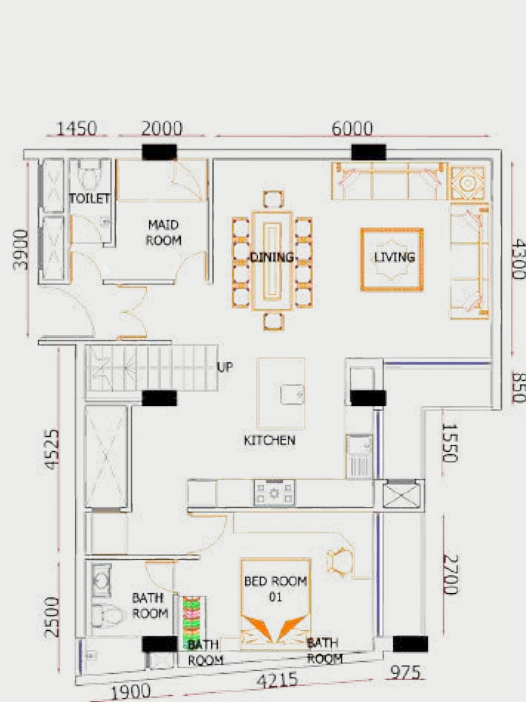
FLOOR PLAN / TYPE 01 LOWER / 01 BED ROOM
